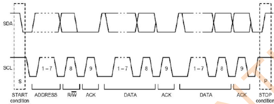
Figure 8 I2C Protocol
