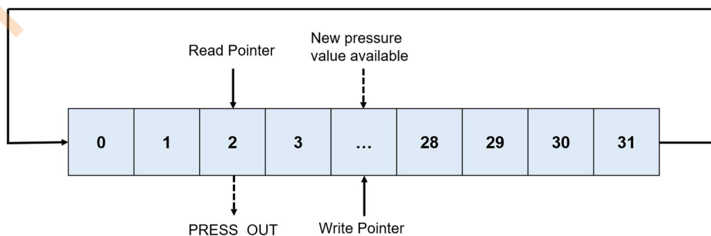
Figure 4: FIFO structure
