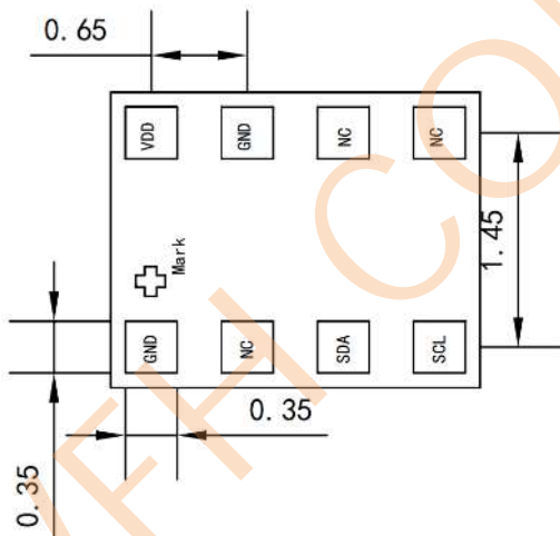
Figure 13: Bottom view
