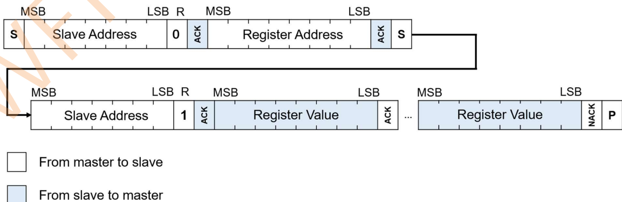
Figure 7: I 2 C read operation
