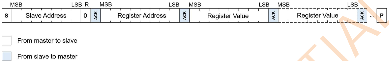
Figure 6: I 2 C write operation
