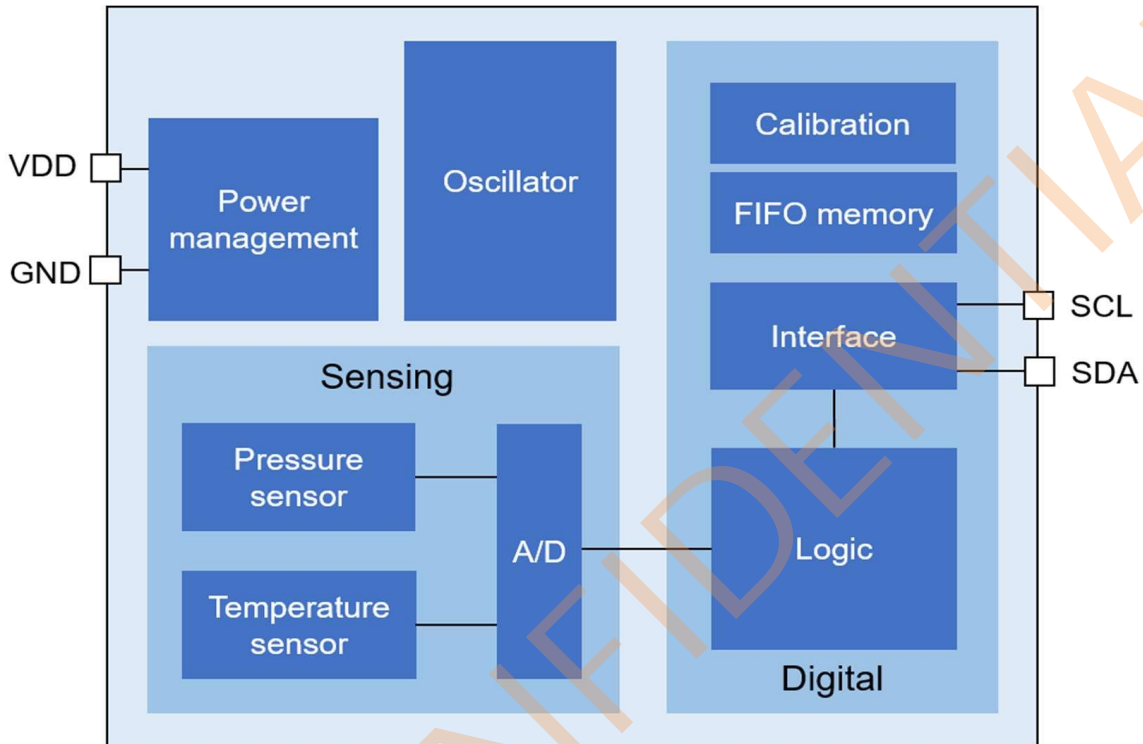
Figure 2: Block diagram of WF286A
