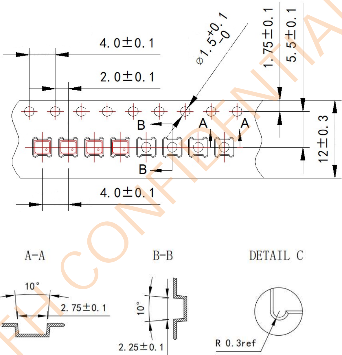
Figure 16: Carrier Tape details
