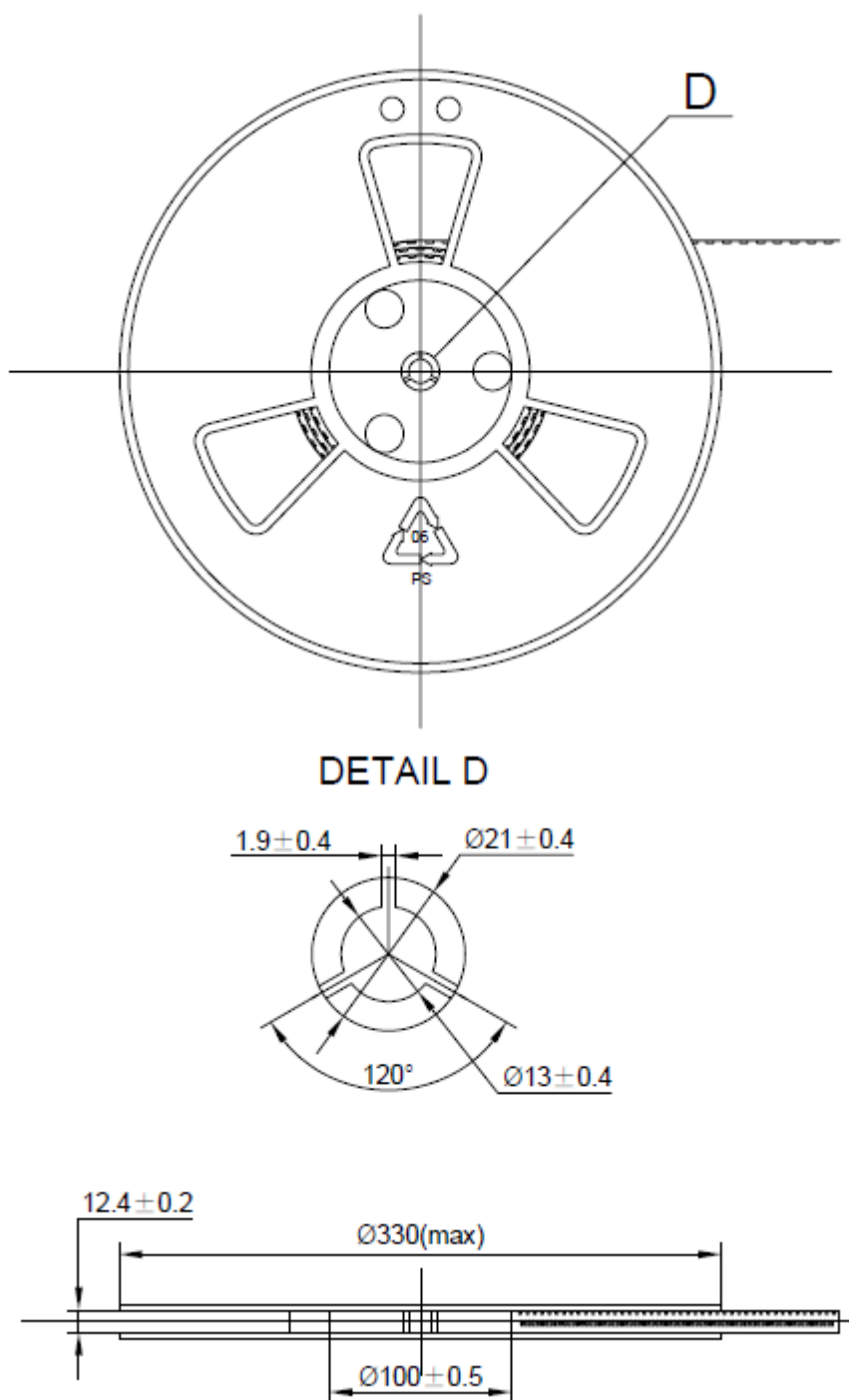
Figure 12: Carrier Tape (2)
