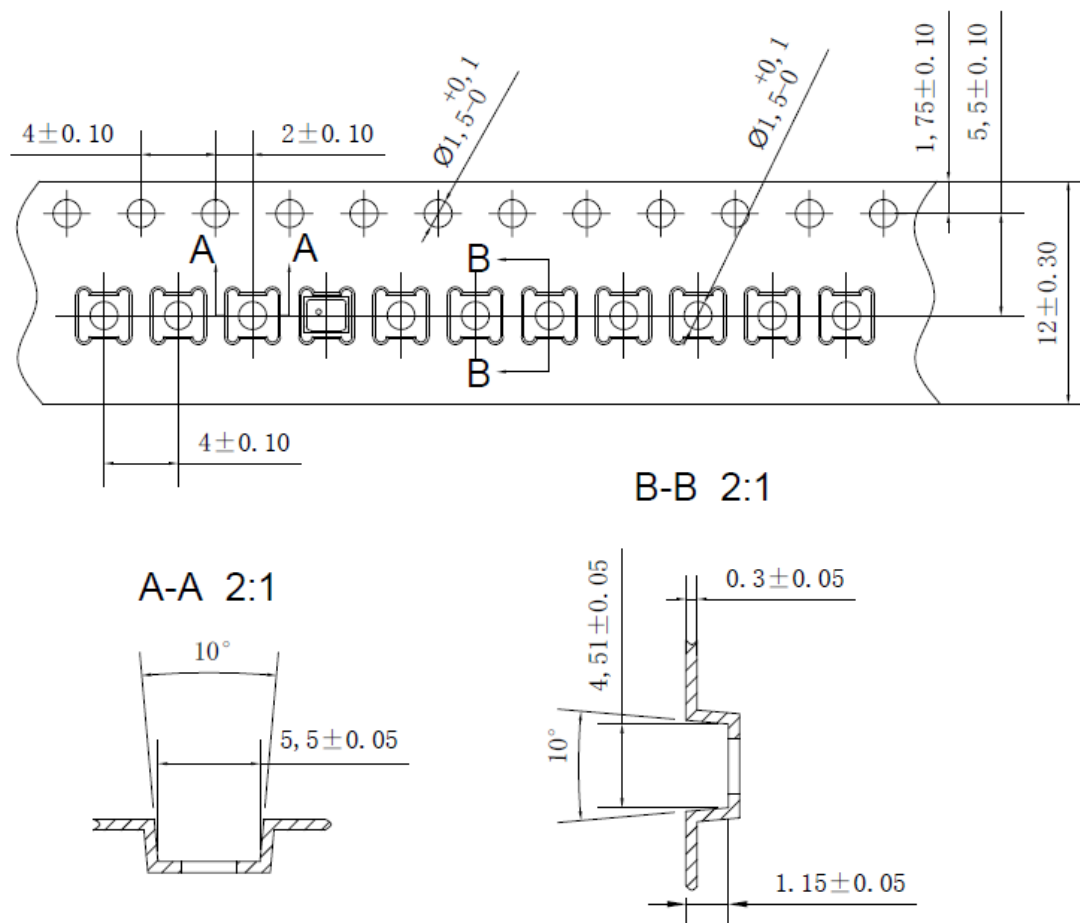
Figure 11: Carrier Tape (1)
